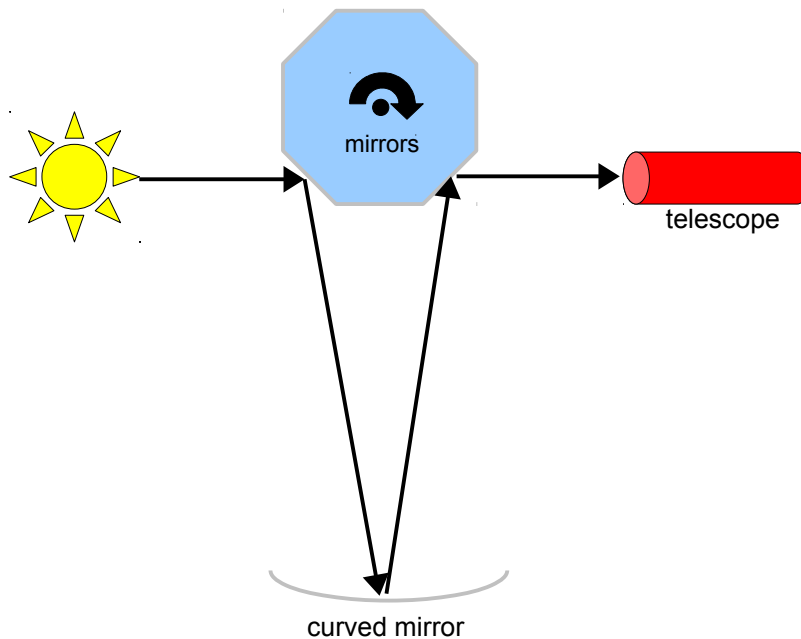
Illustration 3: Michelson's apparatus.
